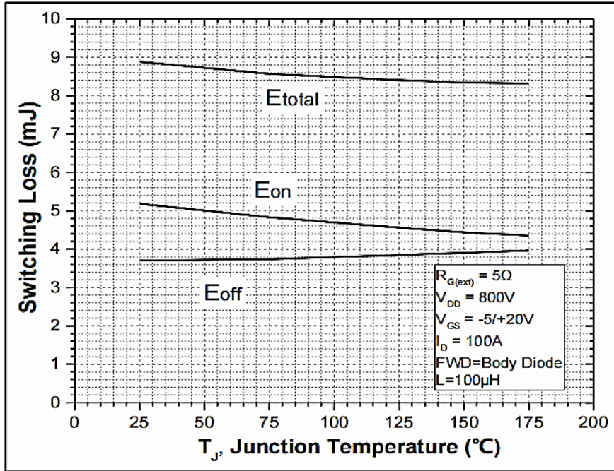
Figure 25. Clamped Inductive Switching Energy vs. T_j
