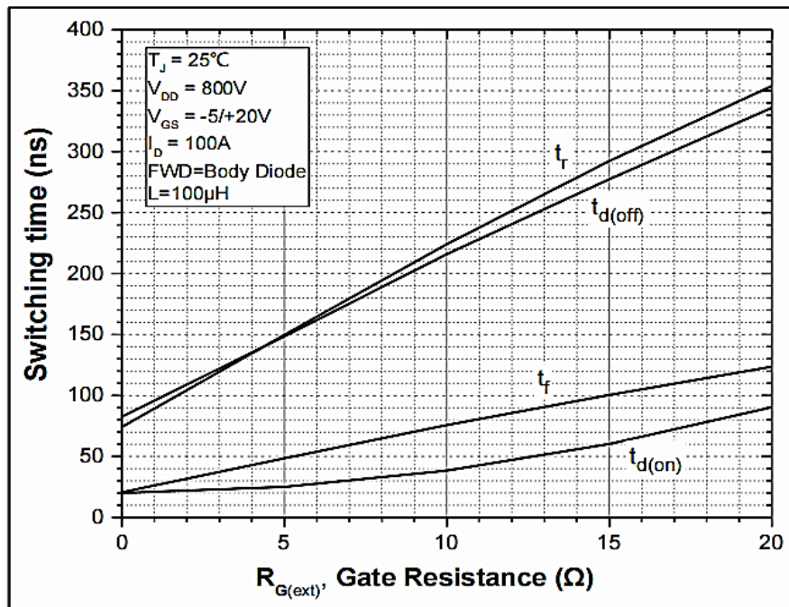
Figure 26. Switching Time vs. R_{G(ext)}
