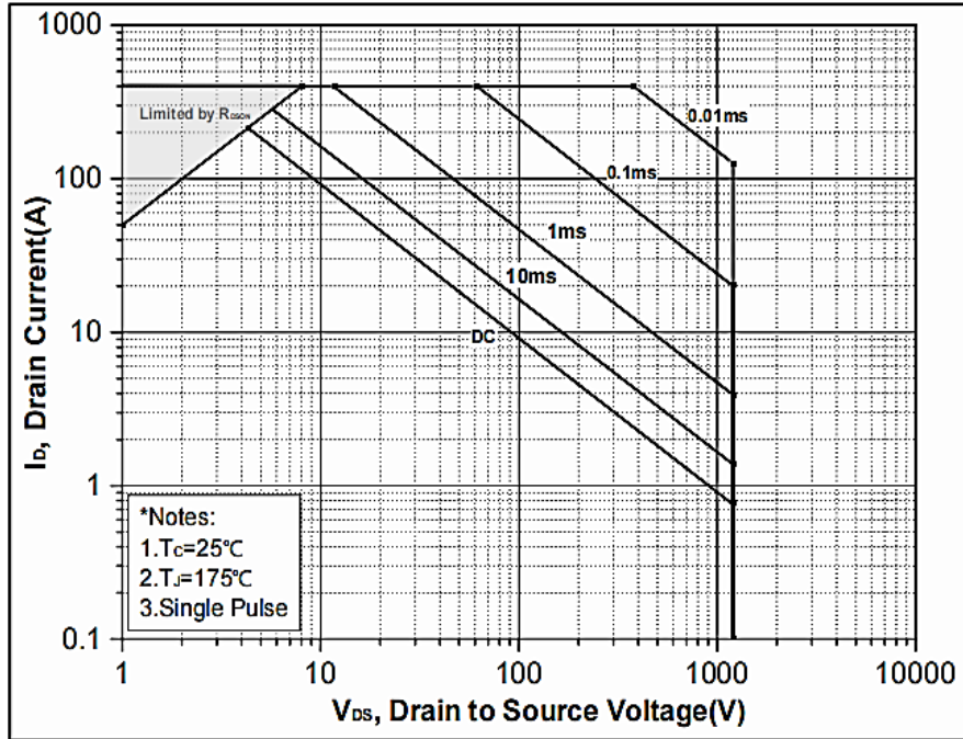
Figure 21. Safe Operating Area
