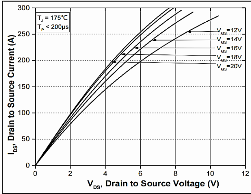
Figure 3. Output Characteristics T_J=175^\circ\text{C}
