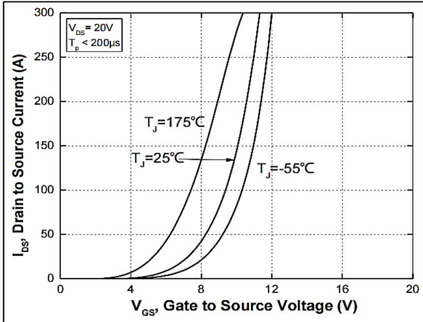
Figure 7. Transfer Characteristic for Various Junction Temperatures
