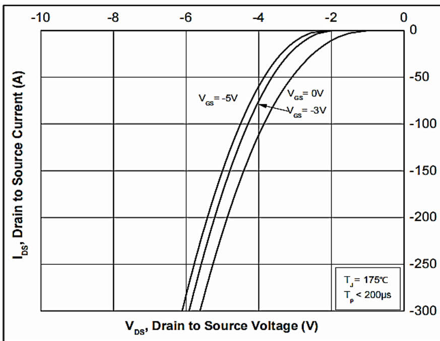
Figure 10. Body Diode Characteristic at 175°C
