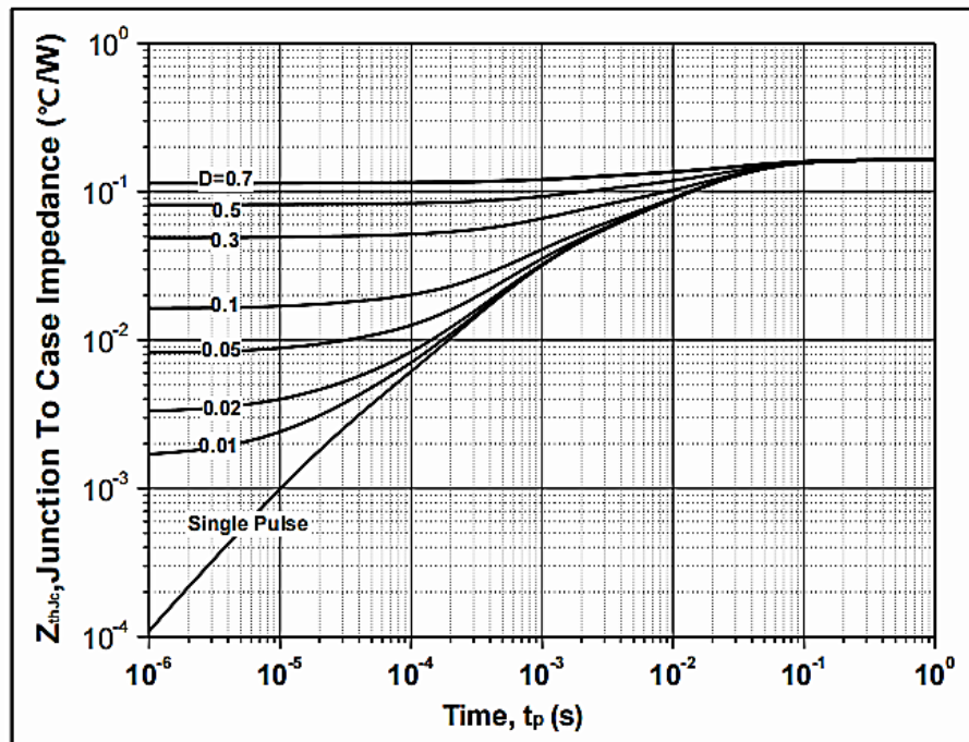
Figure 20. Transient Thermal Impedance (Junction - Case)
