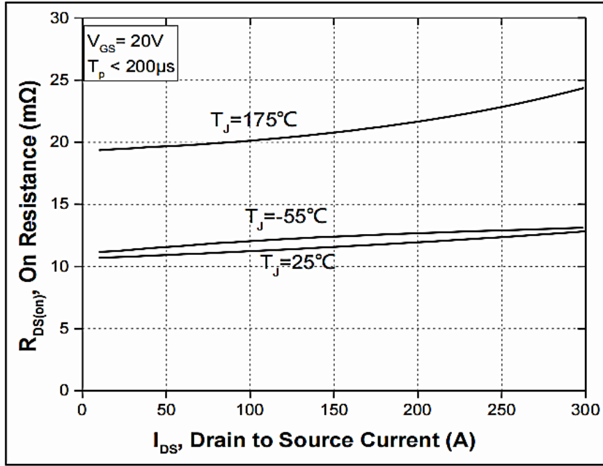
Figure 5. On-Resistance vs. Drain Current For Various Temperatures
