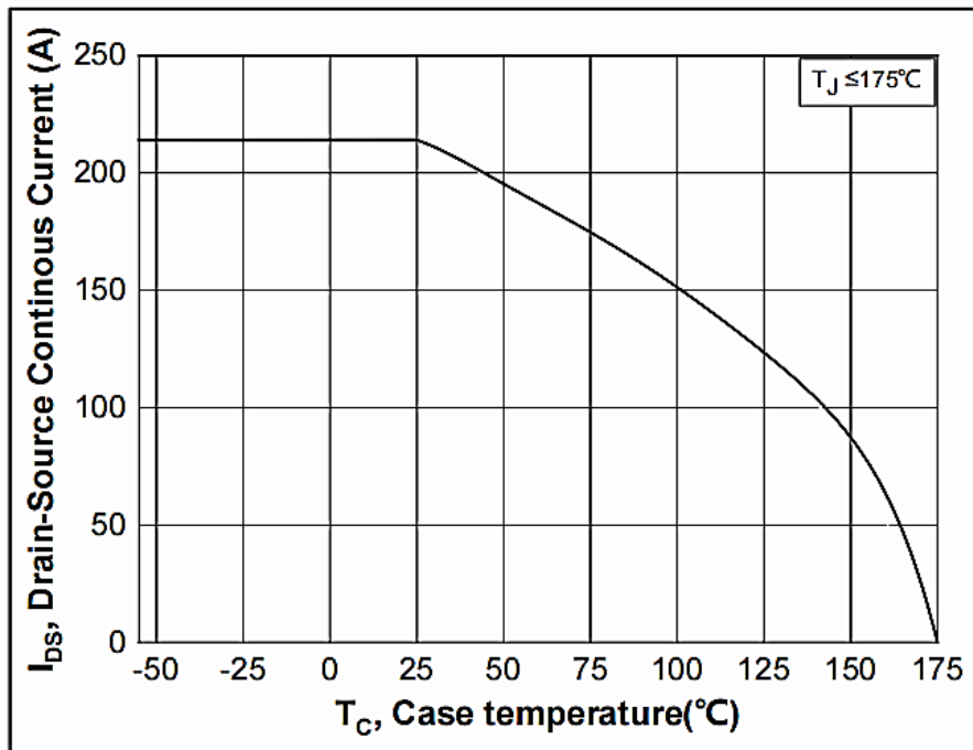
Figure 18. Continuous Drain Current Derating vs. Case Temperature
