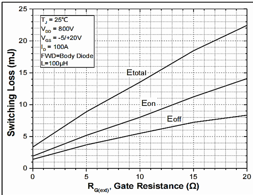
Figure 24. Clamped Inductive Switching Energy vs. R_{G(ext)}
