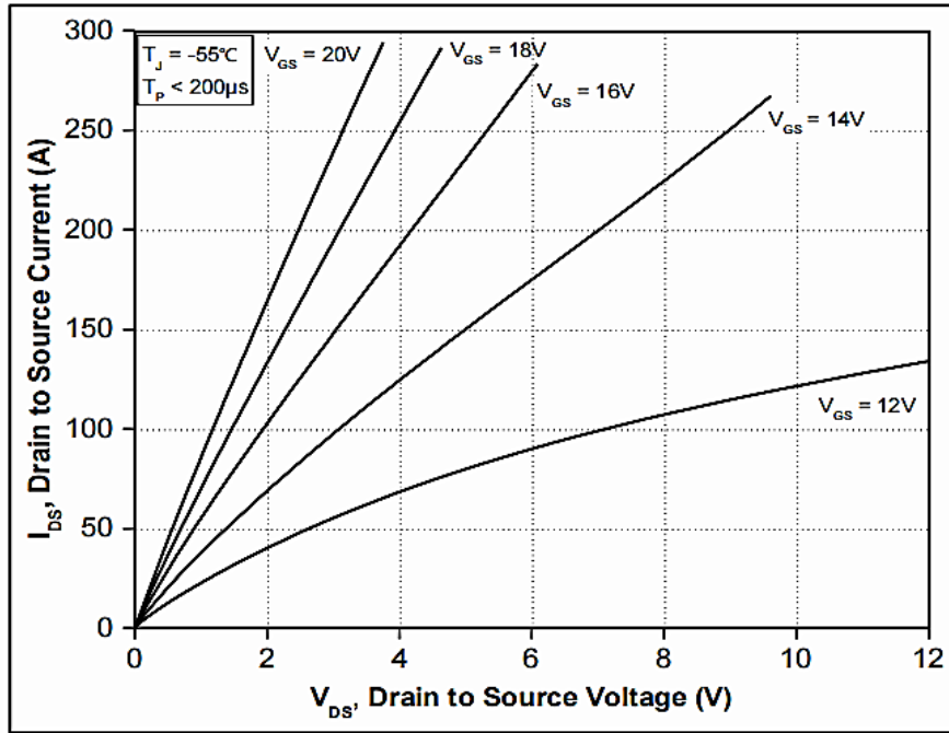
Figure 1. Output Characteristics T_J = -55^\circ\text{C}
